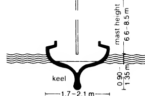
13 Open-keel boat: section
